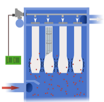
Pulse-Jet Dust Collector during cleaning phase
