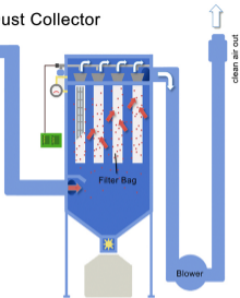
Pulse-Jet Dust Collector
